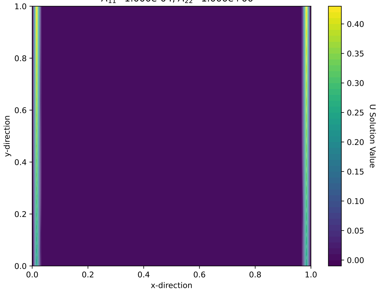
RBF-FD Approximate Solution (Contour): A_{11}=1.000\text{e-}04 , A_{22}=1.000\text{e+}00
